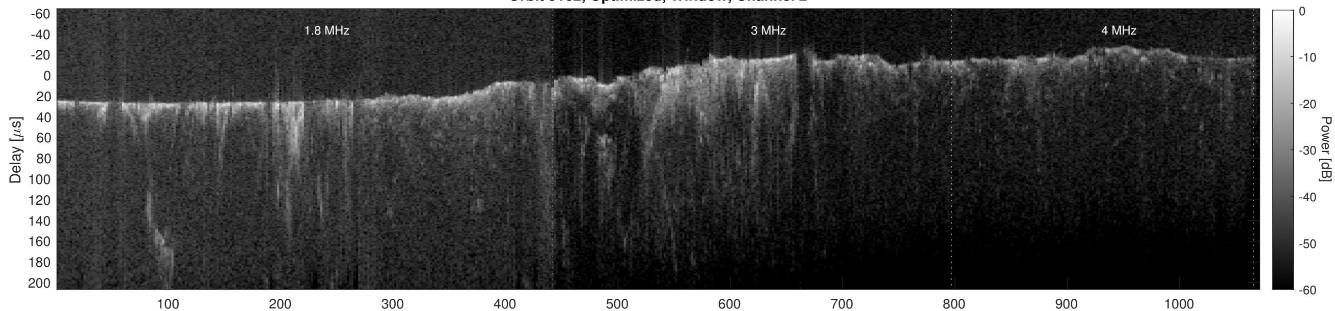
Orbit 9162, Cluttergram
