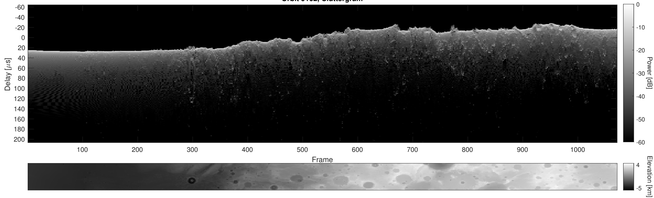
Orbit 9162, Cluttergram
