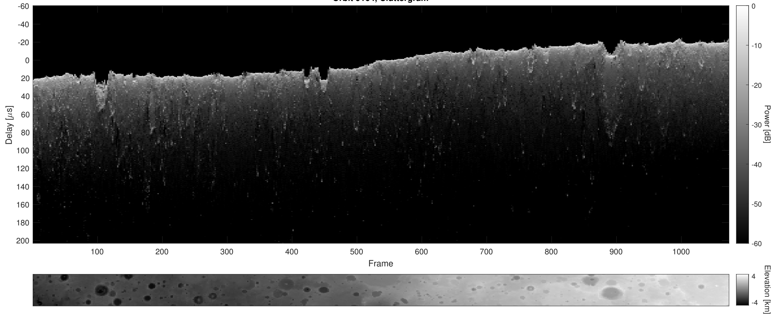
Orbit 9164, Cluttergram
