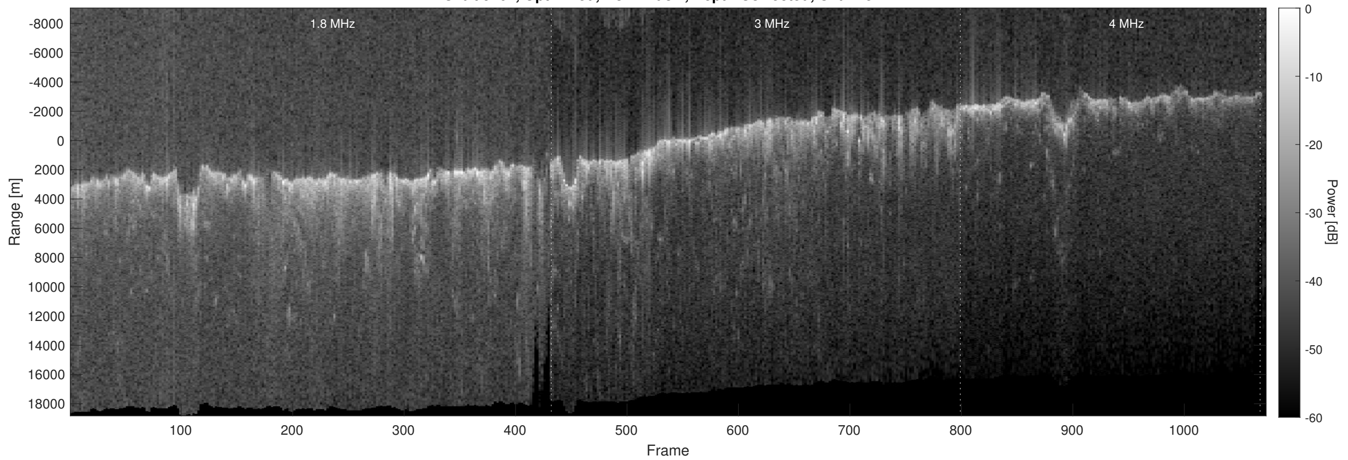
Orbit 9164, Optimized, No Window, Depth-Corrected, Channel 2
