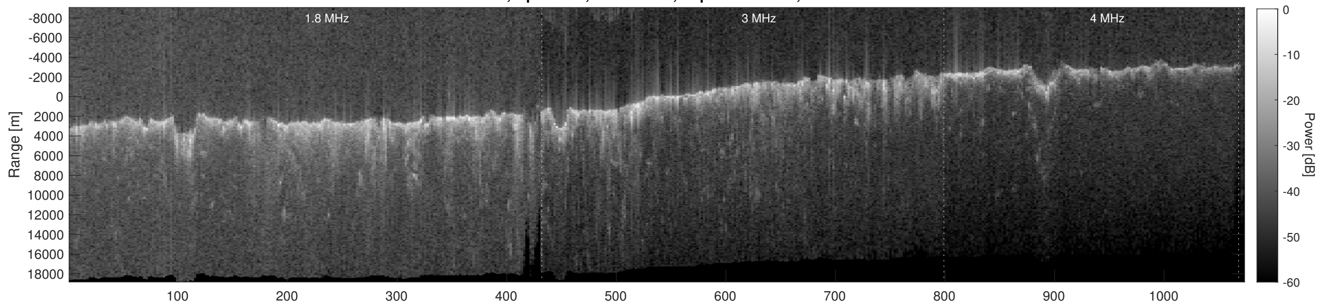
Orbit 9164, Depth-Corrected Cluttergram
