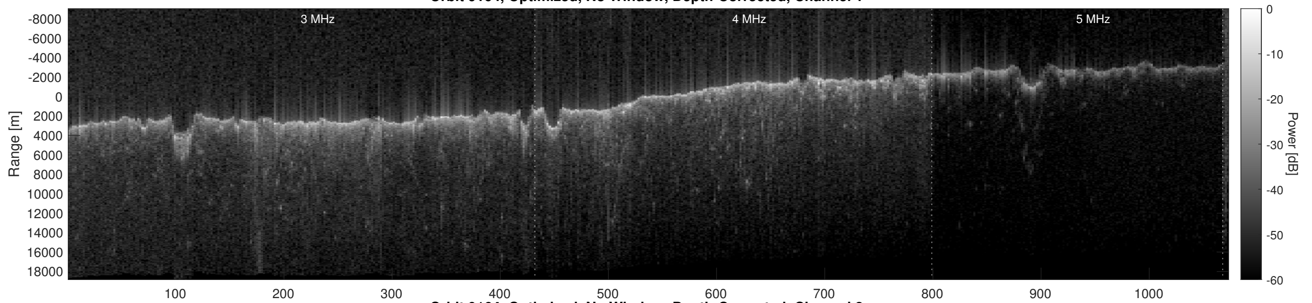
Orbit 9164, Optimized, No Window, Depth-Corrected, Channel 2
