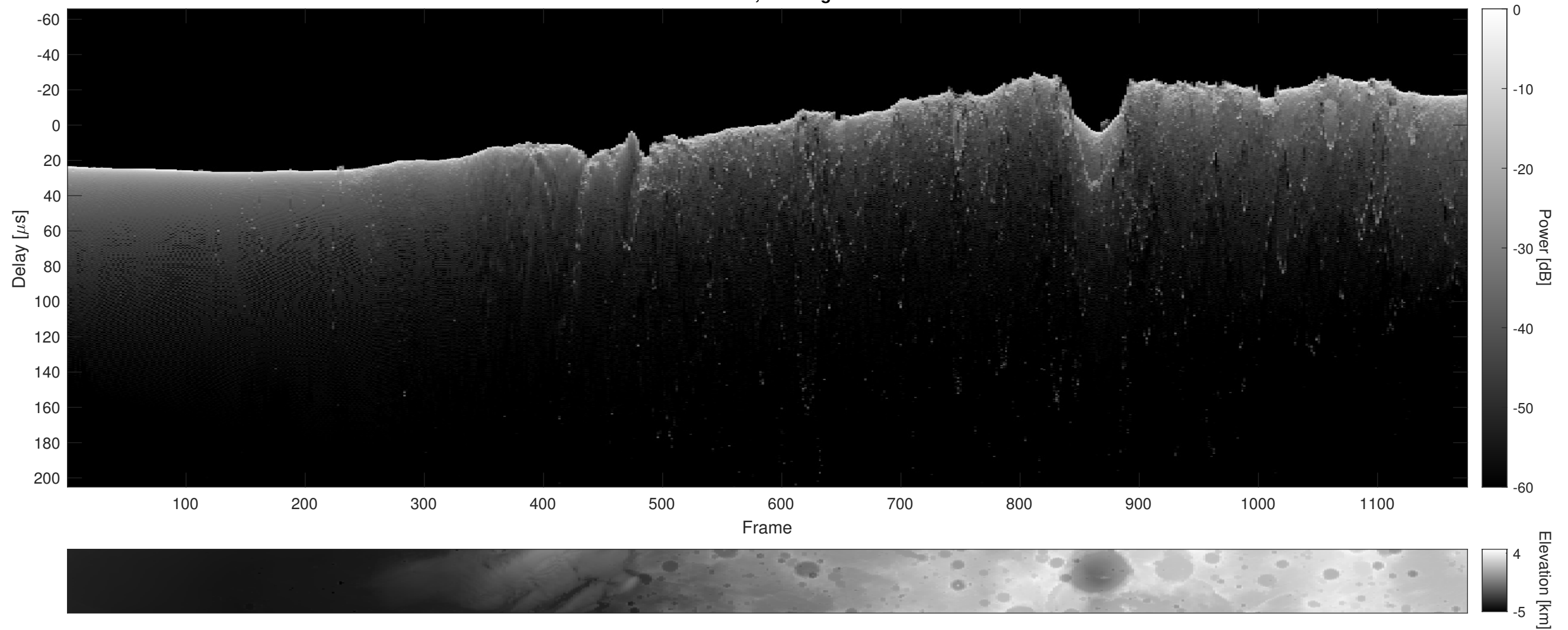
Orbit 9169, Cluttergram
