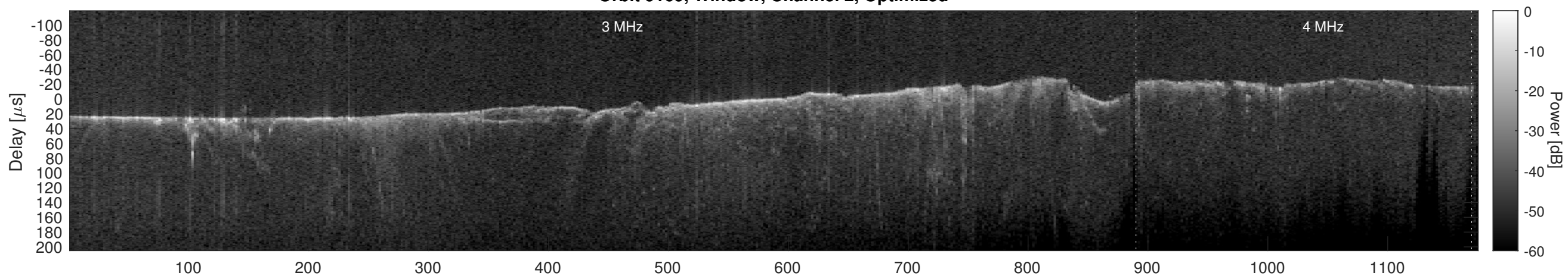
Orbit 9169, Cluttergram
