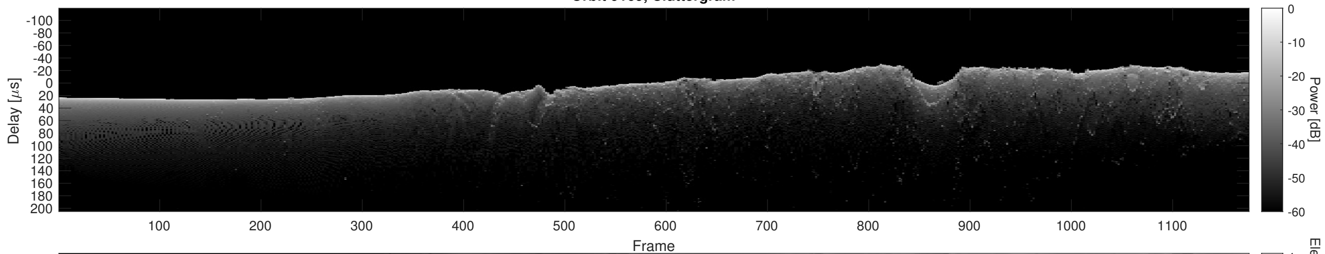
Orbit 9169, Cluttergram
