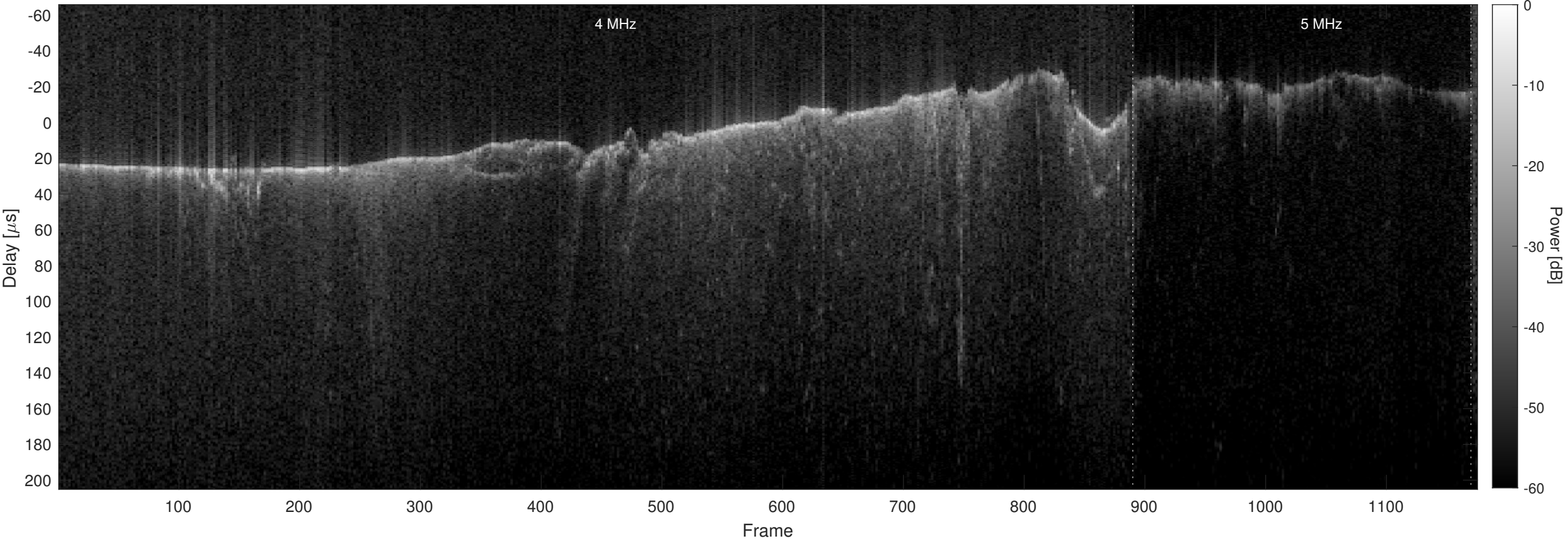
Orbit 9169, Optimized, No Window, Channel 2
