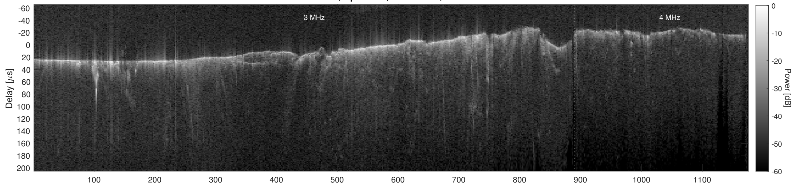
Orbit 9169, Cluttergram
