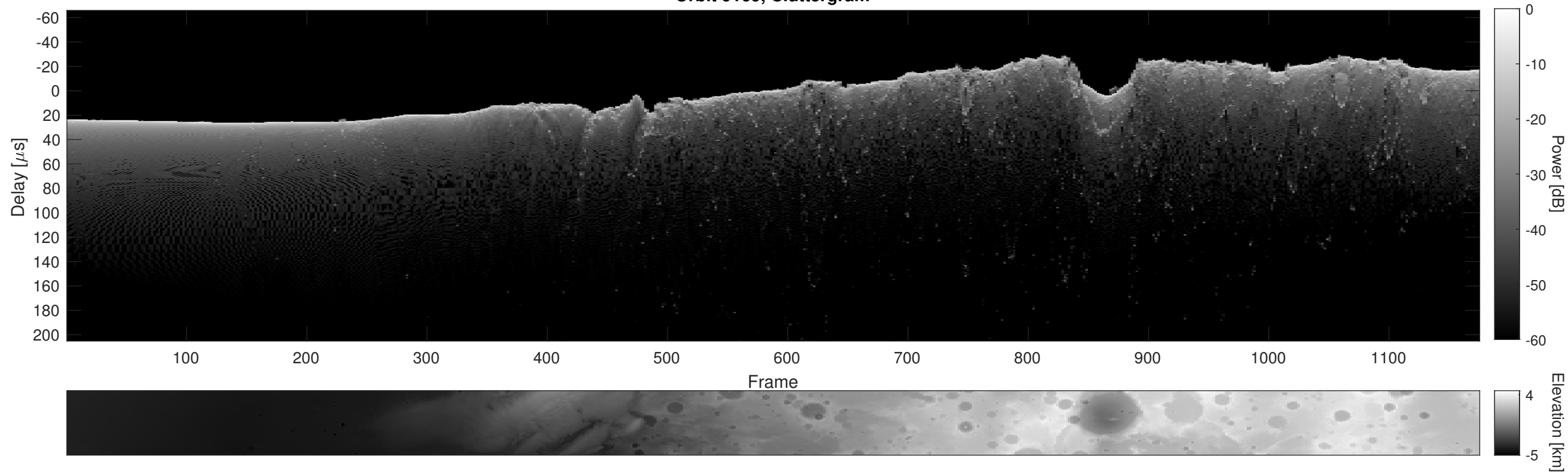
Orbit 9169, Cluttergram
