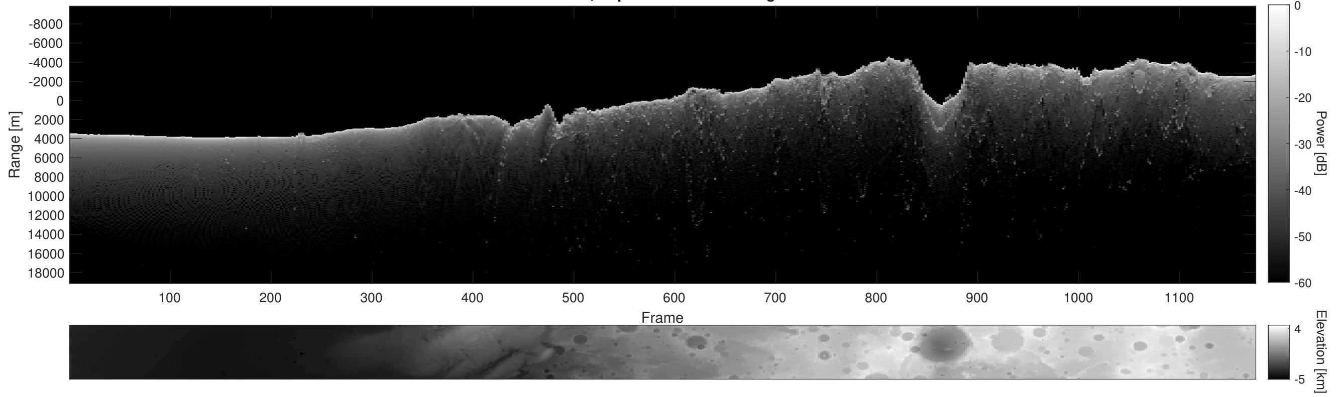
Orbit 9169, Depth-Corrected Cluttergram
