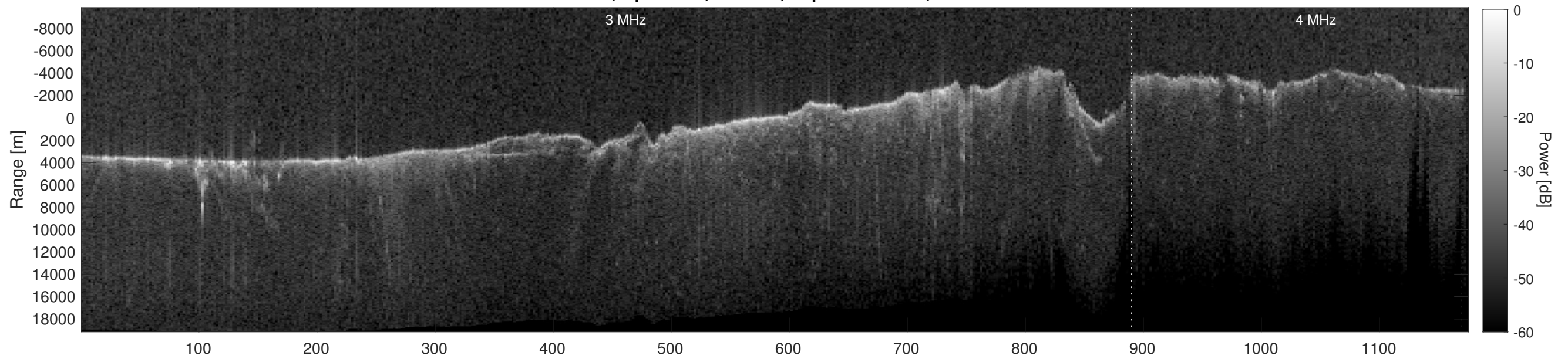
Orbit 9169, Depth-Corrected Cluttergram
