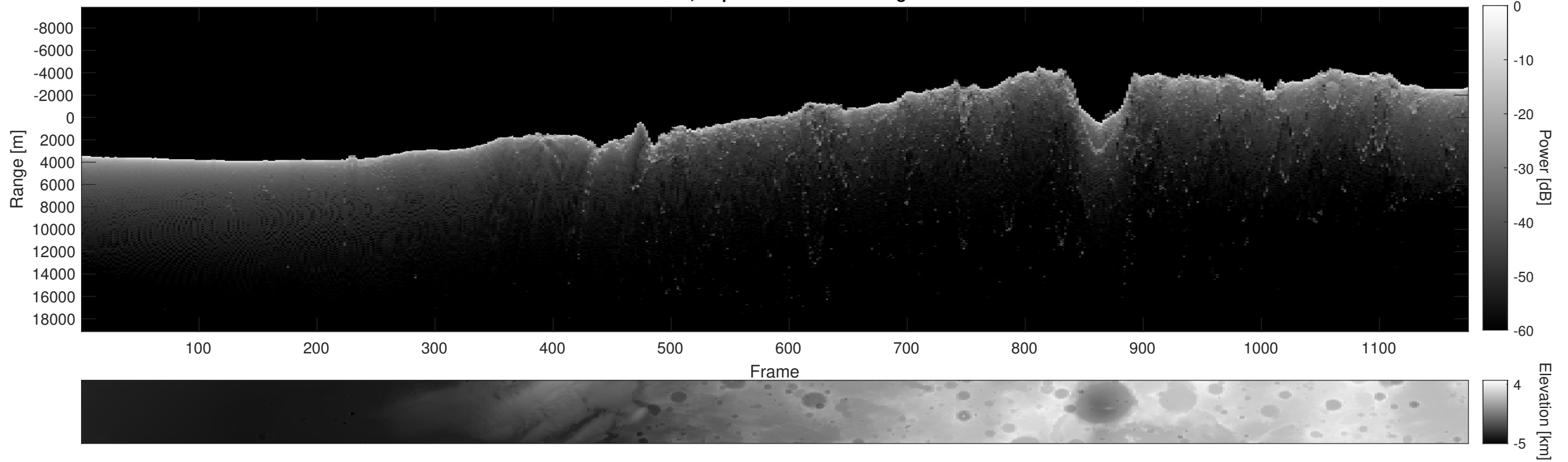
Orbit 9169, Depth-Corrected Cluttergram
