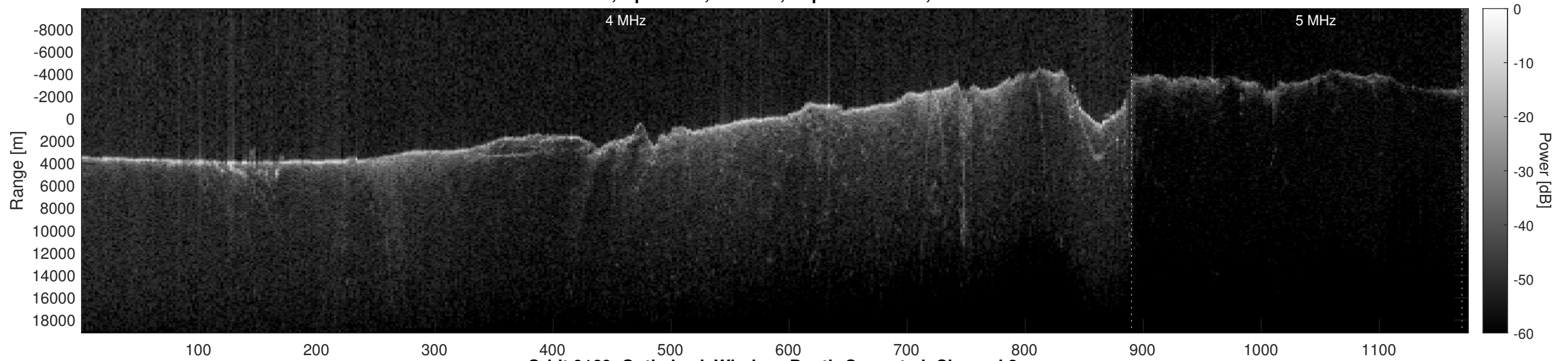
Orbit 9169, Optimized, Window, Depth-Corrected, Channel 2
