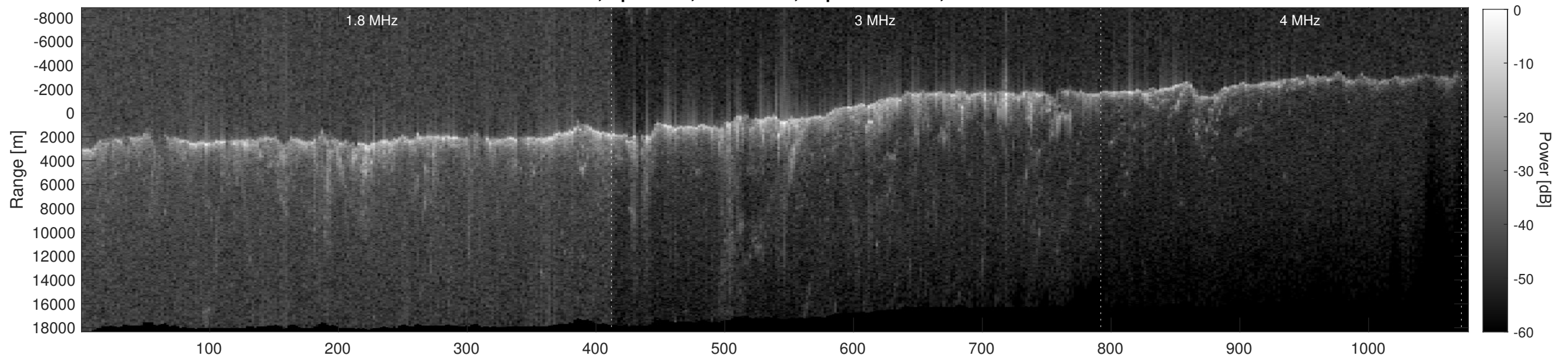
Orbit 9171, Depth-Corrected Cluttergram
