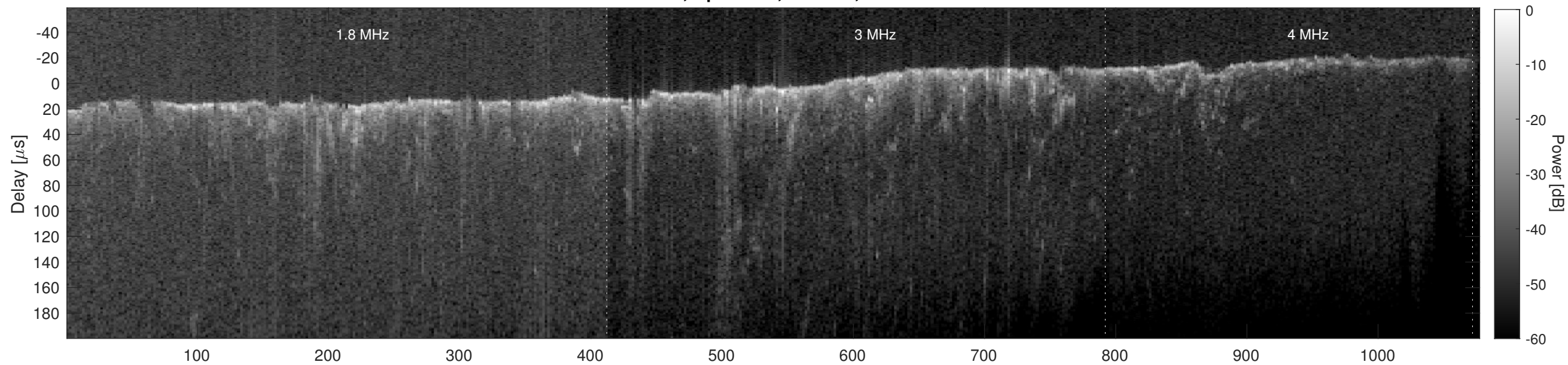
Orbit 9171, Cluttergram
