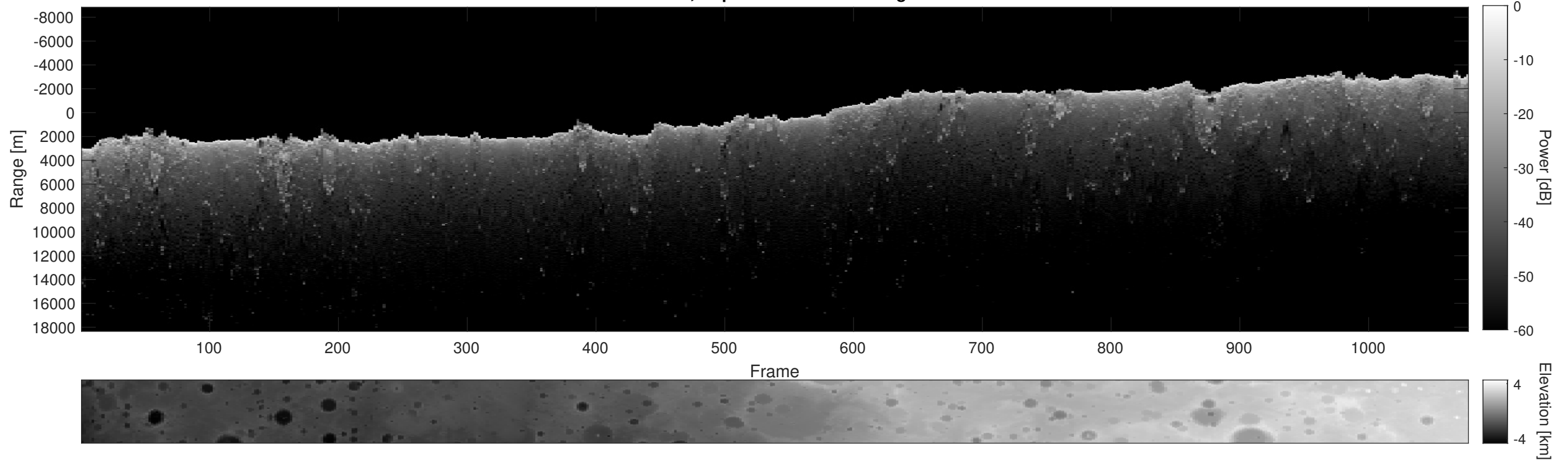
Orbit 9171, Depth-Corrected Cluttergram
