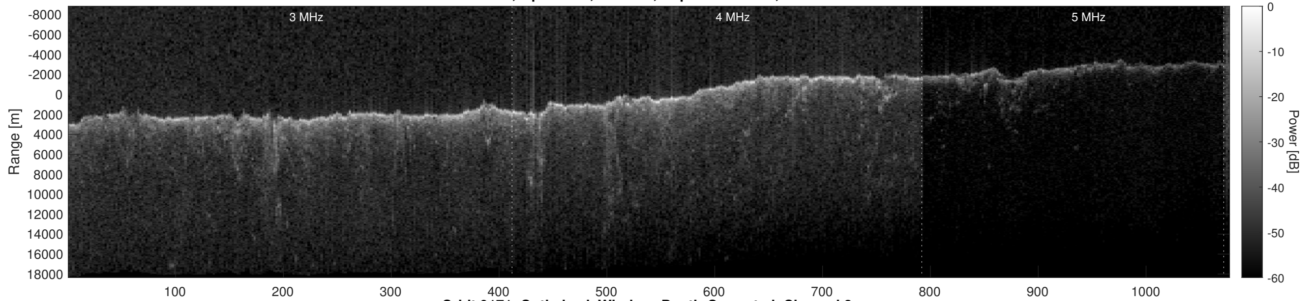
Orbit 9171, Optimized, Window, Depth-Corrected, Channel 2
