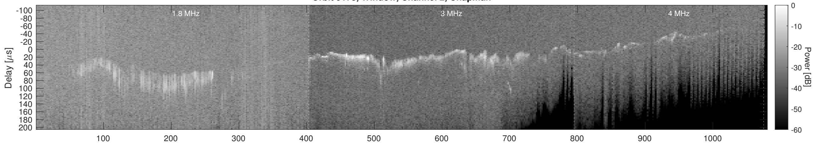
Orbit 9173, Window, Channel 2, Optimized
