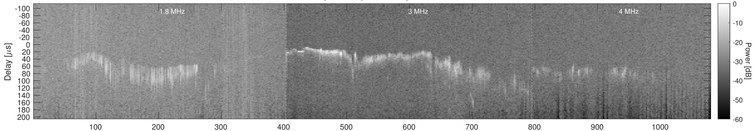
Orbit 9173, Window, Channel 2, Chapman
