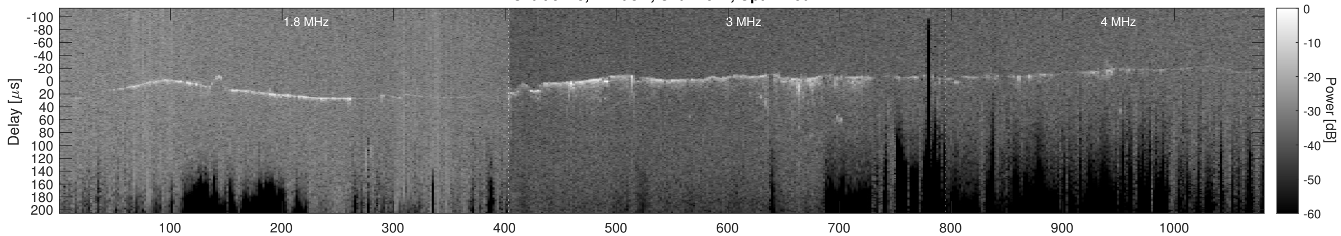
Orbit 9173, Cluttergram
