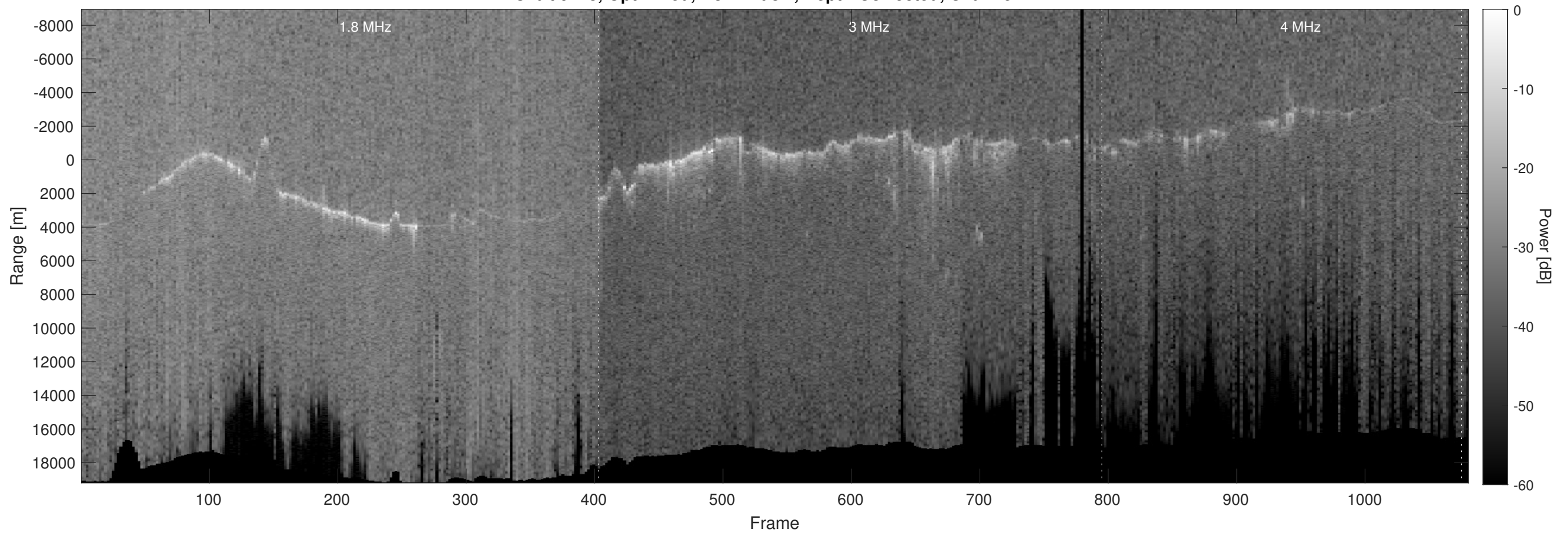
Orbit 9173, Optimized, No Window, Depth-Corrected, Channel 2
