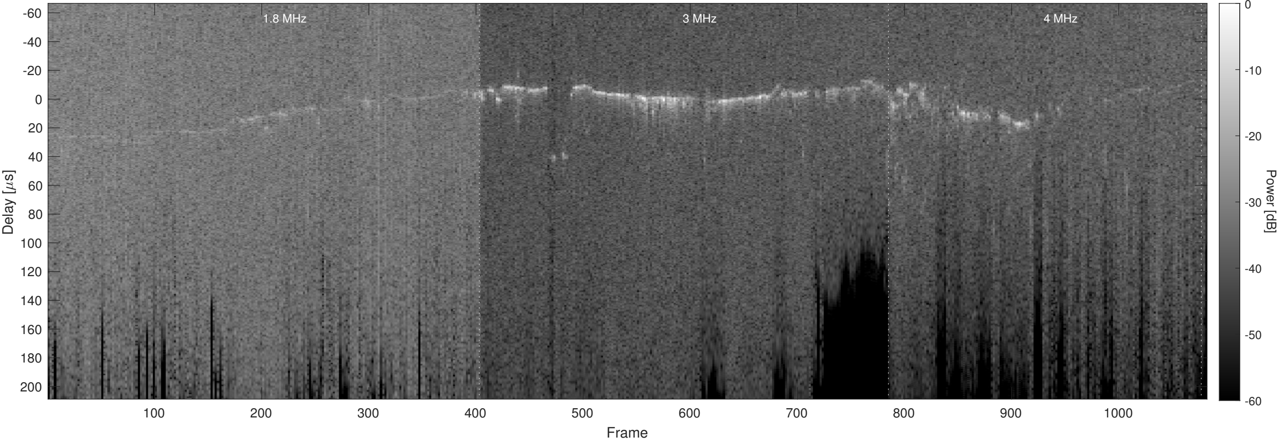
Orbit 9175, Optimized, No Window, Channel 2
