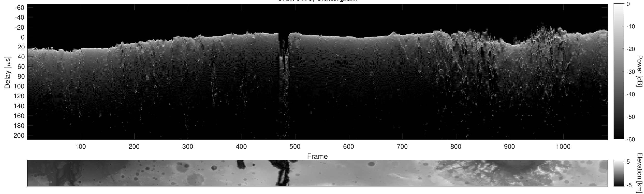
Orbit 9175, Cluttergram
