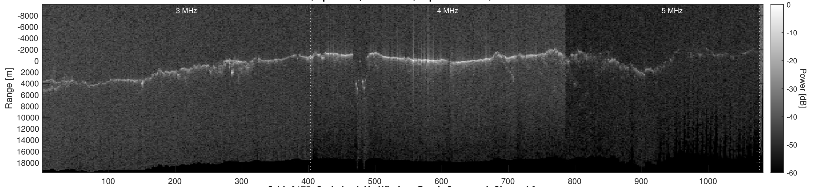
Orbit 9175, Optimized, No Window, Depth-Corrected, Channel 2
