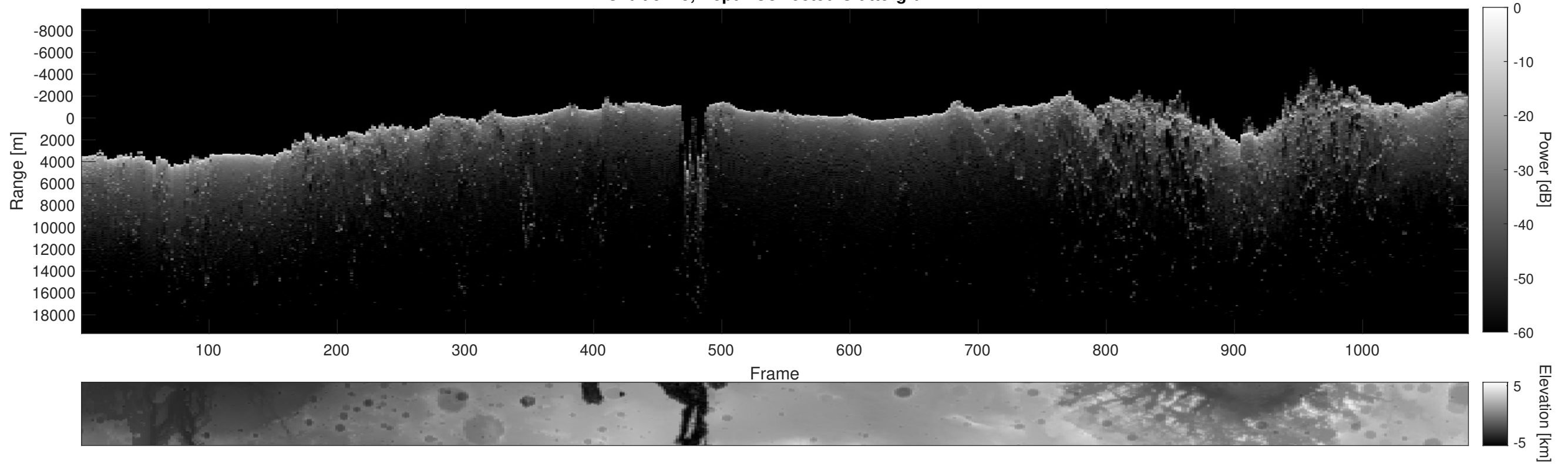
Orbit 9175, Depth-Corrected Cluttergram
