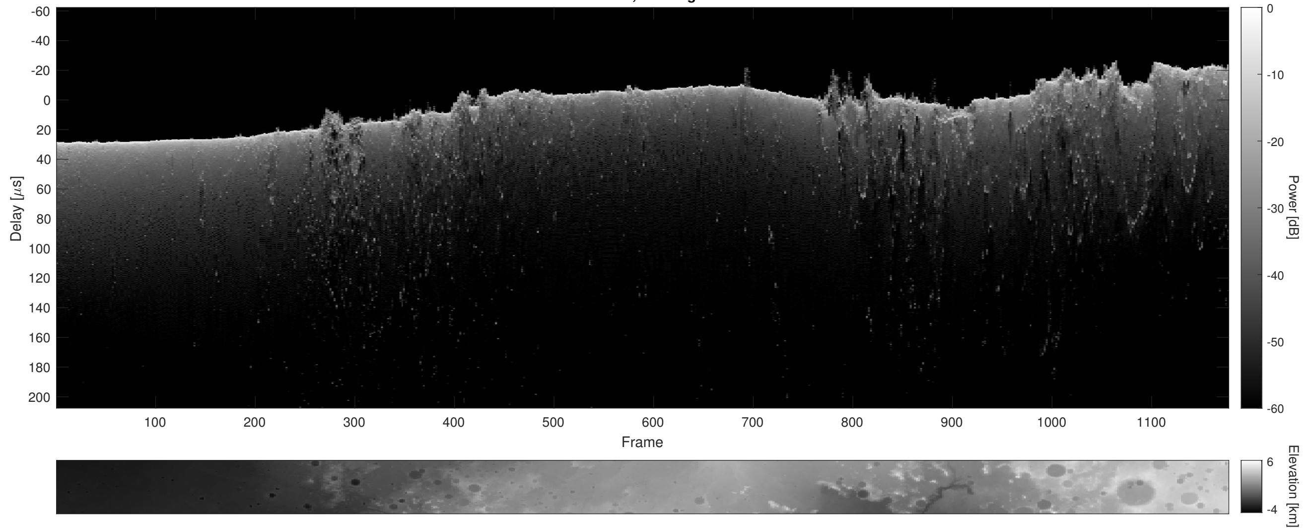
Orbit 9177, Cluttergram
