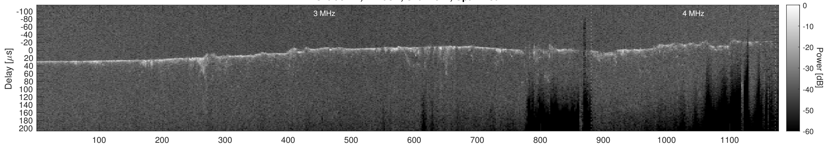
Orbit 9177, Cluttergram
