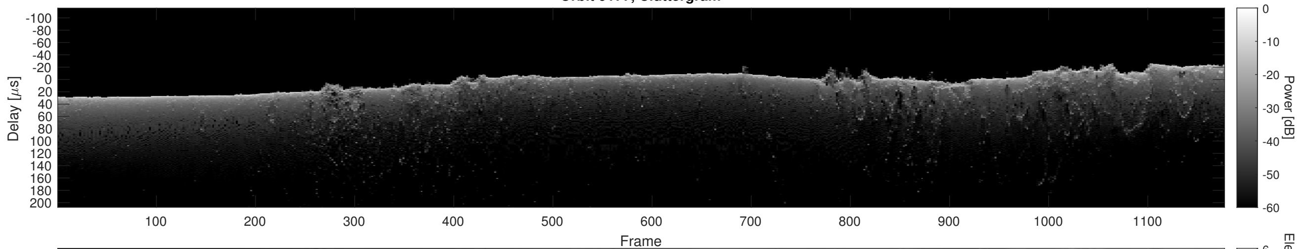
Orbit 9177, Cluttergram
