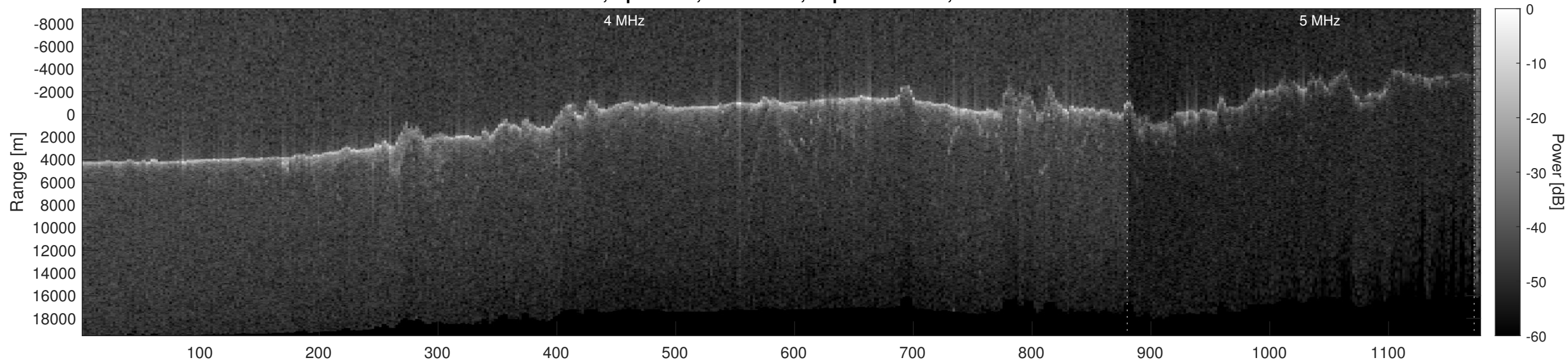
Orbit 9177, Optimized, No Window, Depth-Corrected, Channel 2
