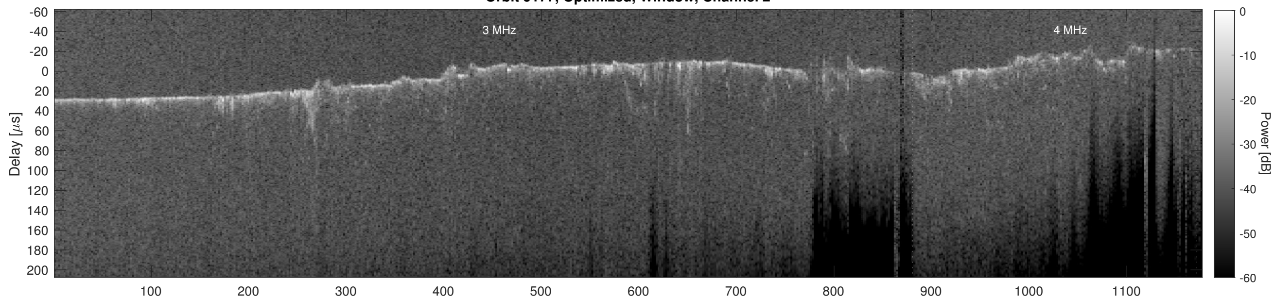
Orbit 9177, Cluttergram
