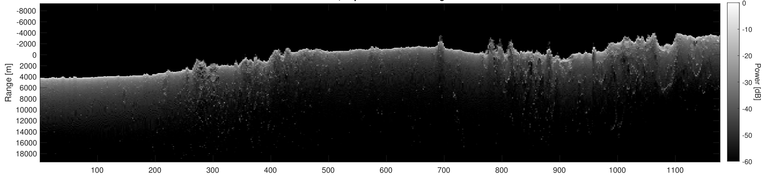
Orbit 9177, Depth-Corrected Cluttergram
