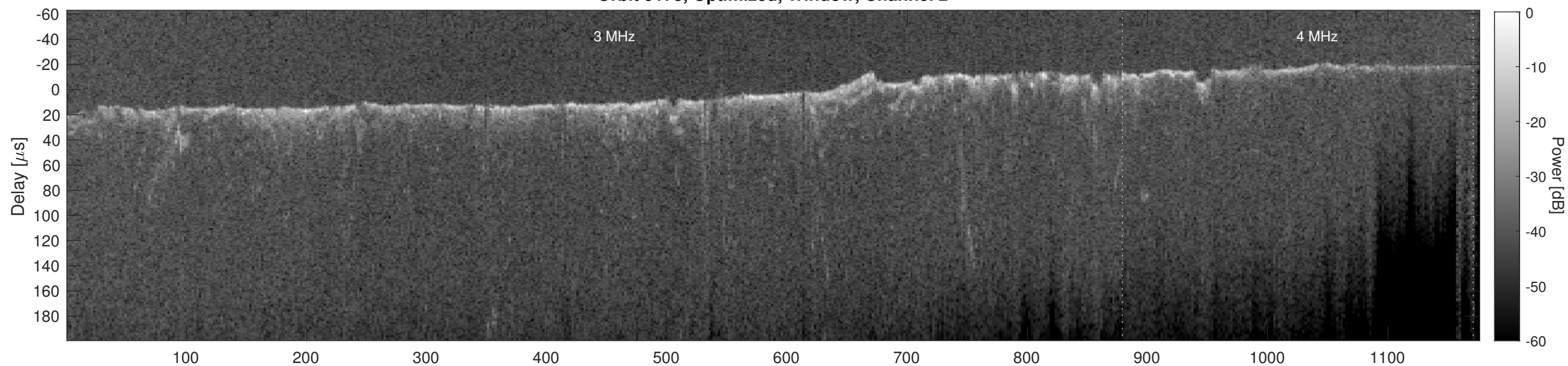
Orbit 9178, Cluttergram
