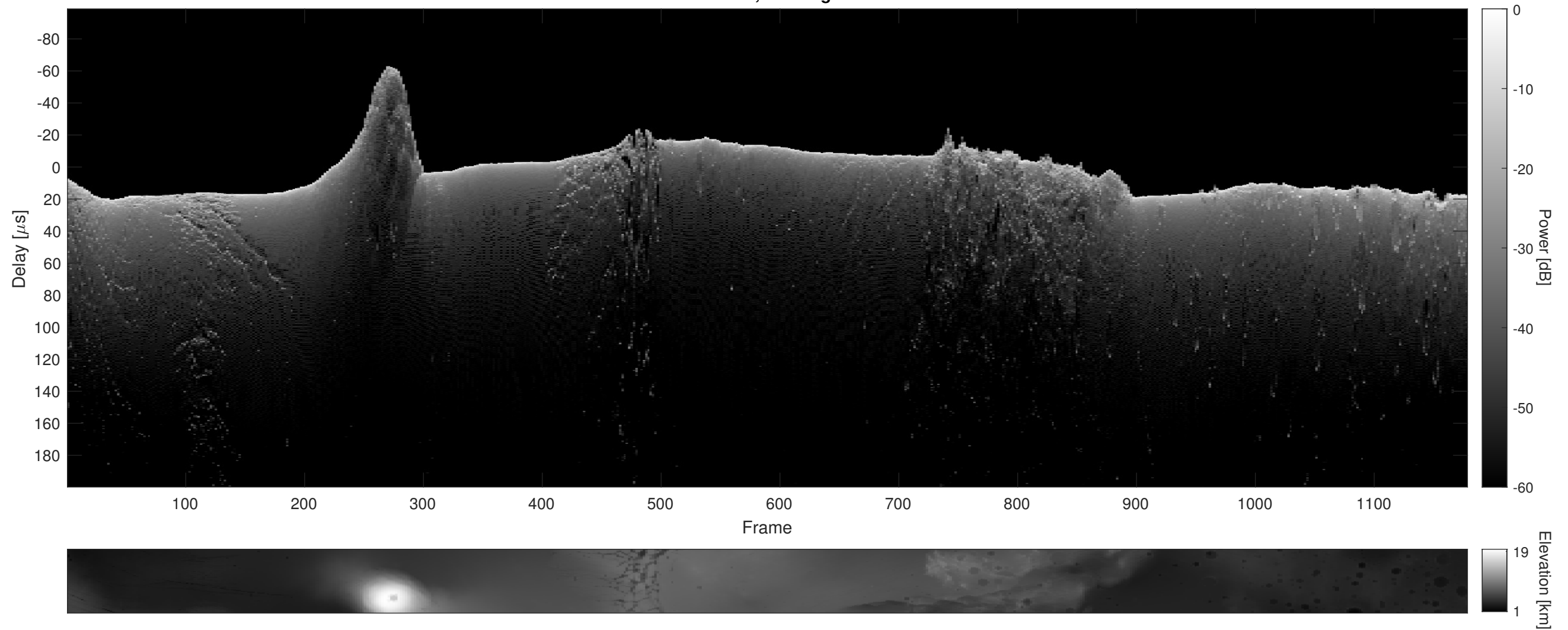
Orbit 9179, Cluttergram
