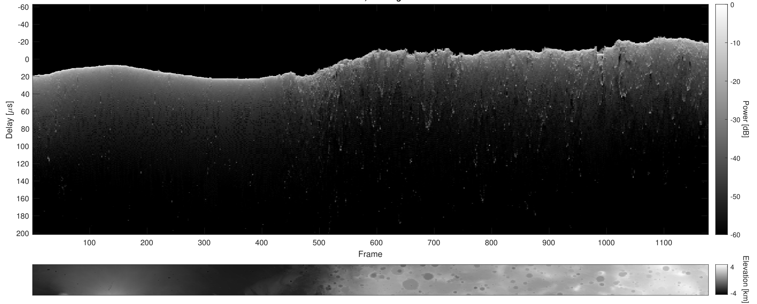
Orbit 9180, Cluttergram
