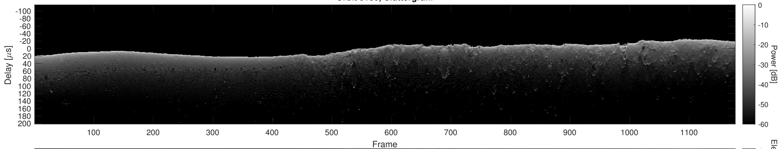
Orbit 9180, Cluttergram
