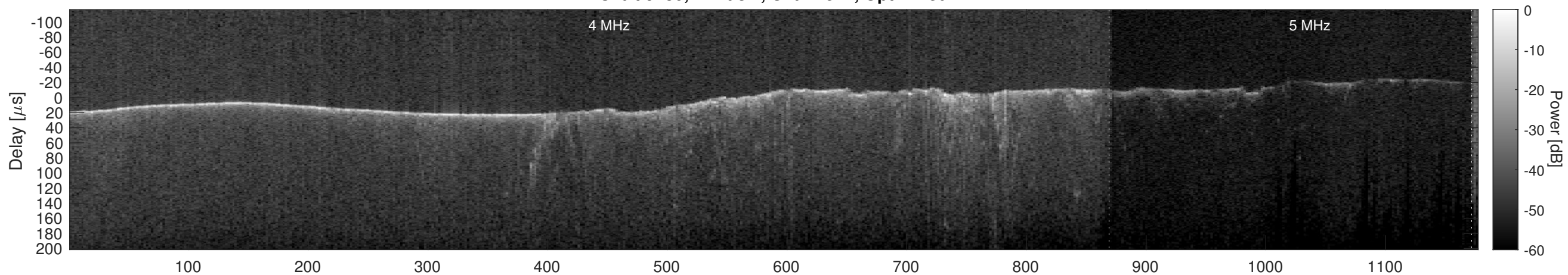
Orbit 9180, Cluttergram
