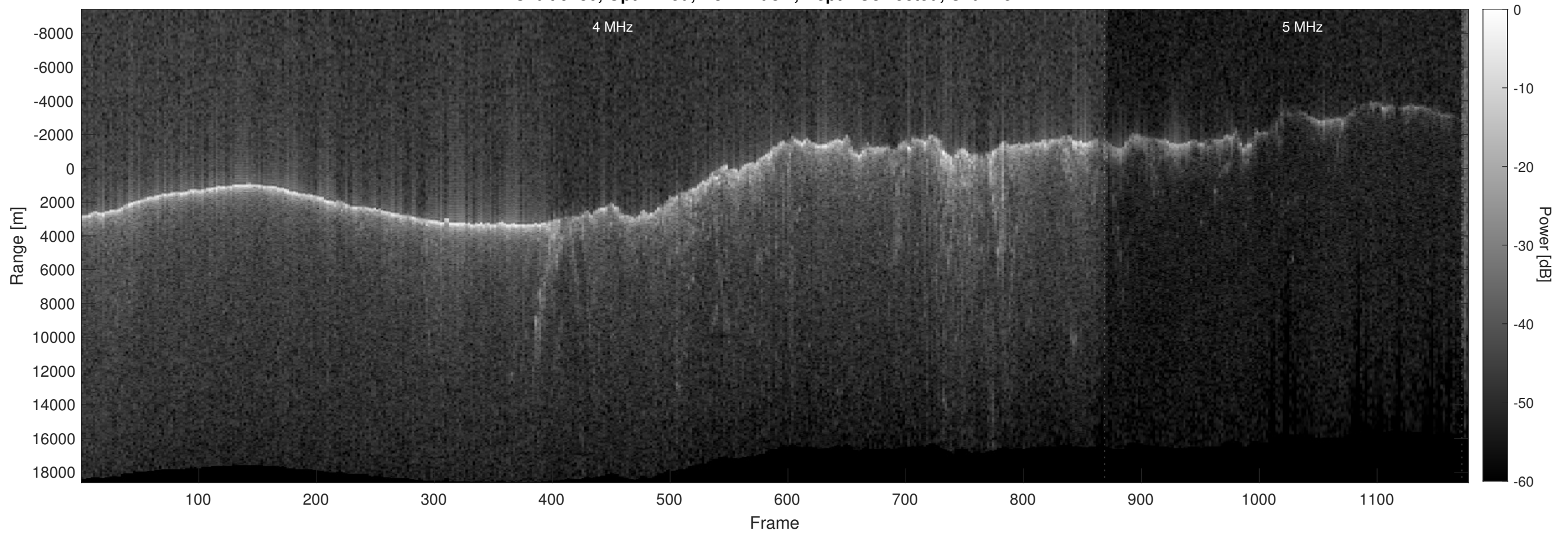
Orbit 9180, Optimized, No Window, Depth-Corrected, Channel 2
