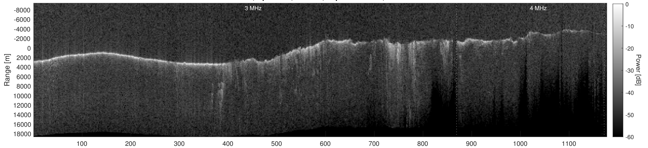
Orbit 9180, Depth-Corrected Cluttergram
