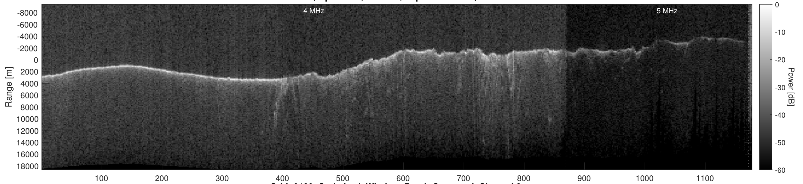
Orbit 9180, Optimized, Window, Depth-Corrected, Channel 2
