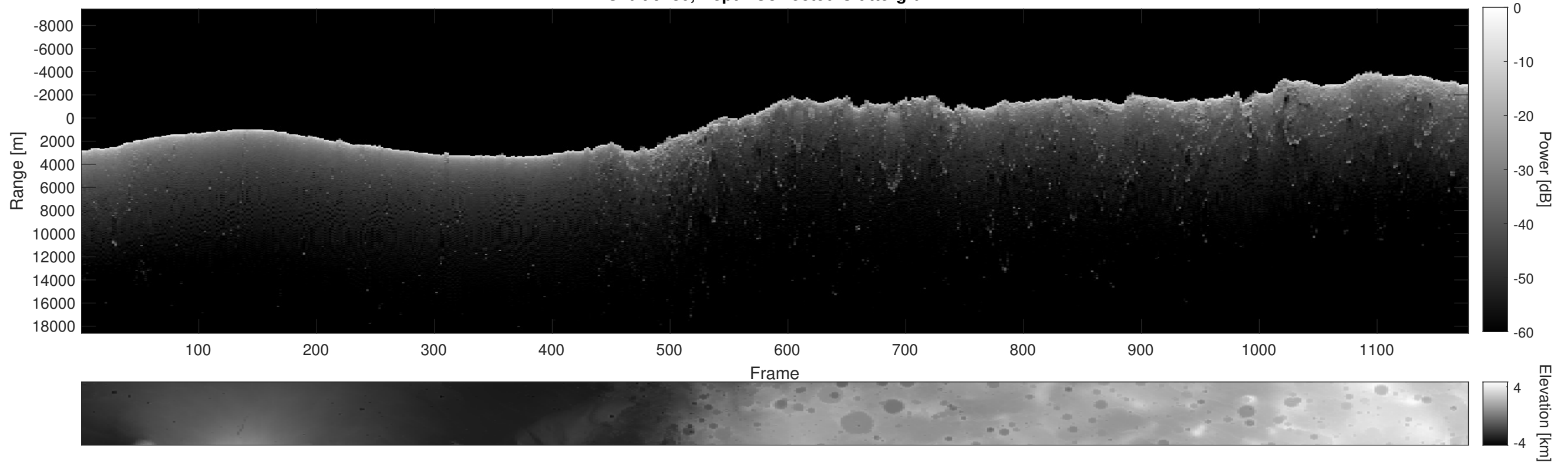
Orbit 9180, Depth-Corrected Cluttergram
