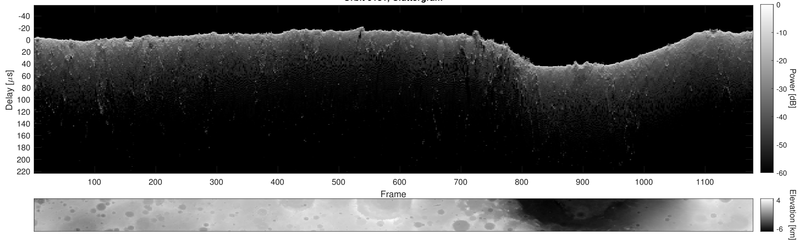
Orbit 9181, Cluttergram
