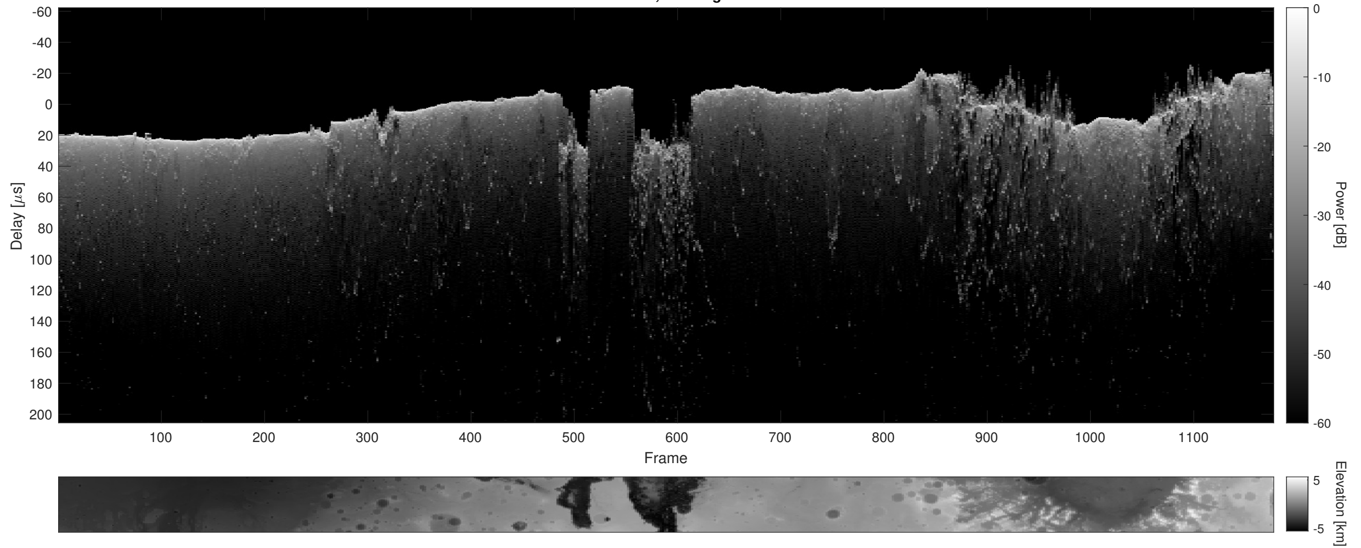
Orbit 9182, Cluttergram
