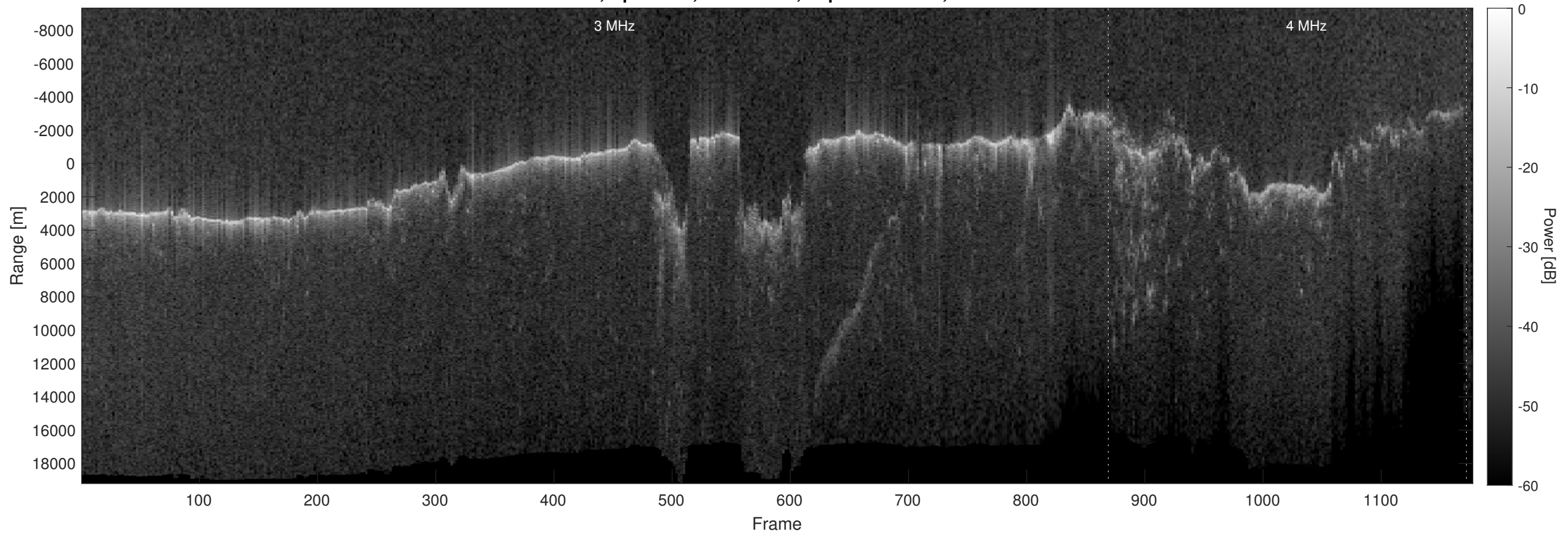
Orbit 9182, Optimized, No Window, Depth-Corrected, Channel 2
