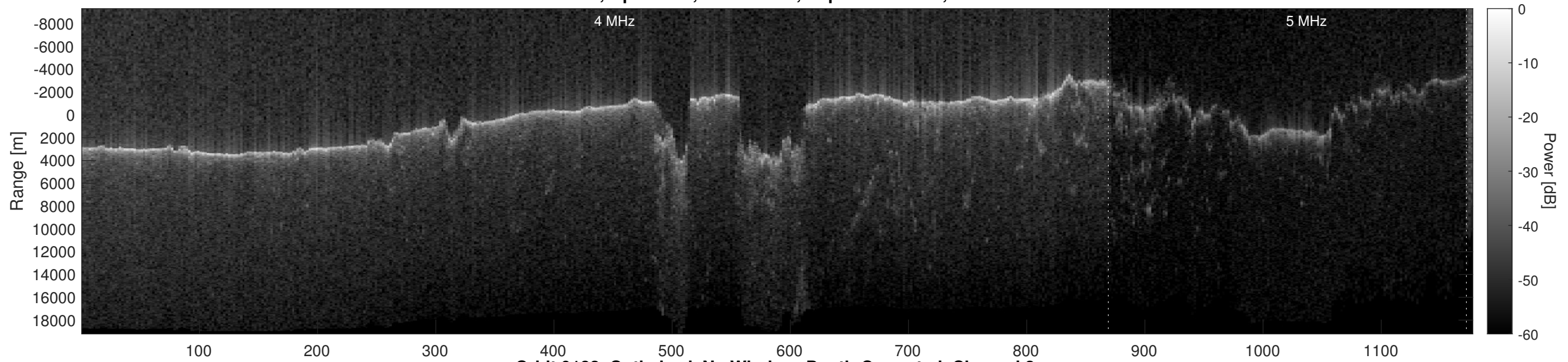
Orbit 9182, Optimized, No Window, Depth-Corrected, Channel 2
