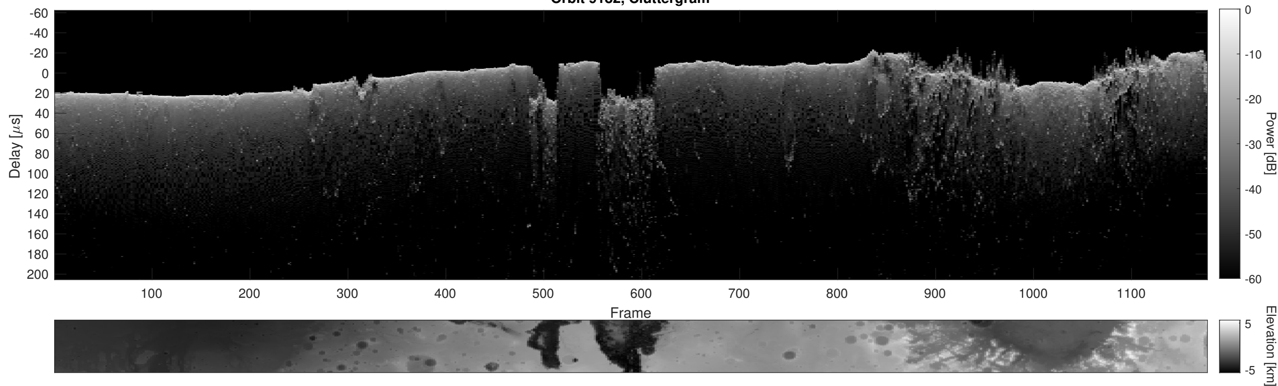
Orbit 9182, Cluttergram
