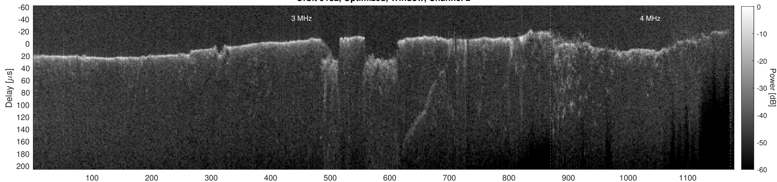
Orbit 9182, Cluttergram
