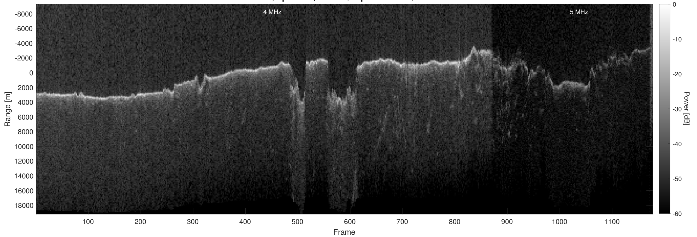
Orbit 9182, Optimized, Window, Depth-Corrected, Channel 2
