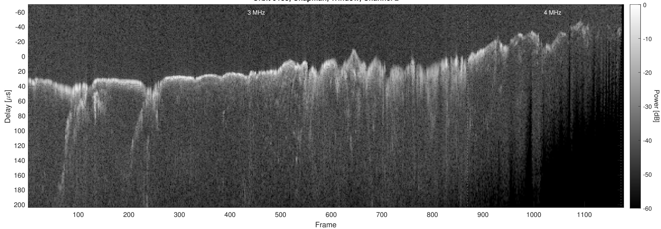
Orbit 9183, Chapman, Window, Channel 2
