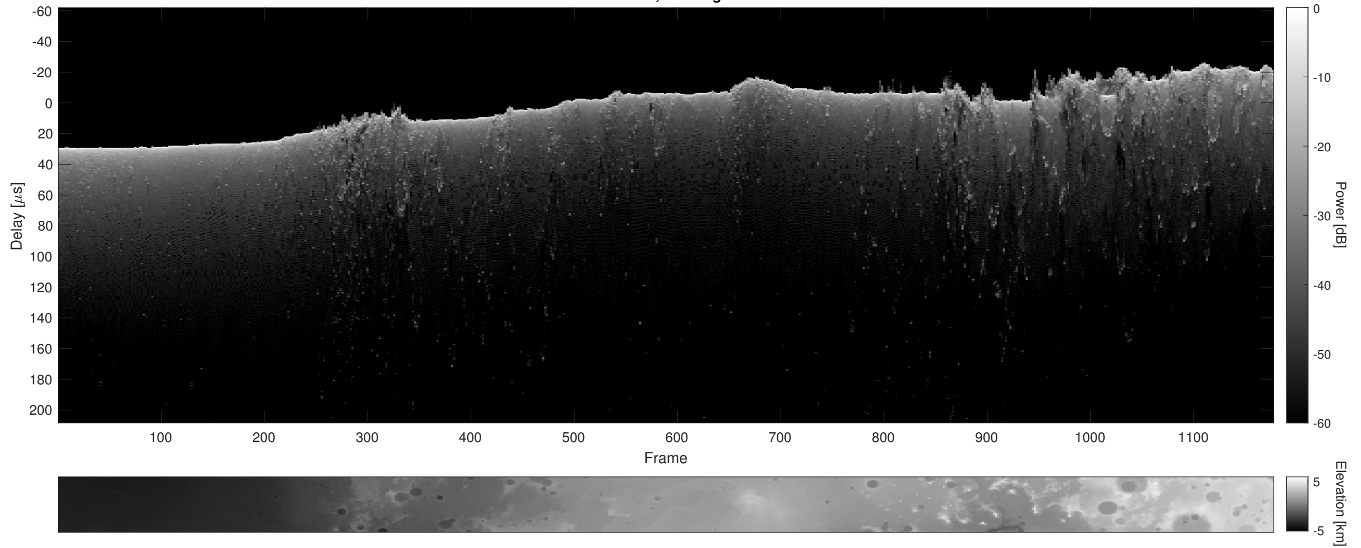
Orbit 9184, Cluttergram
