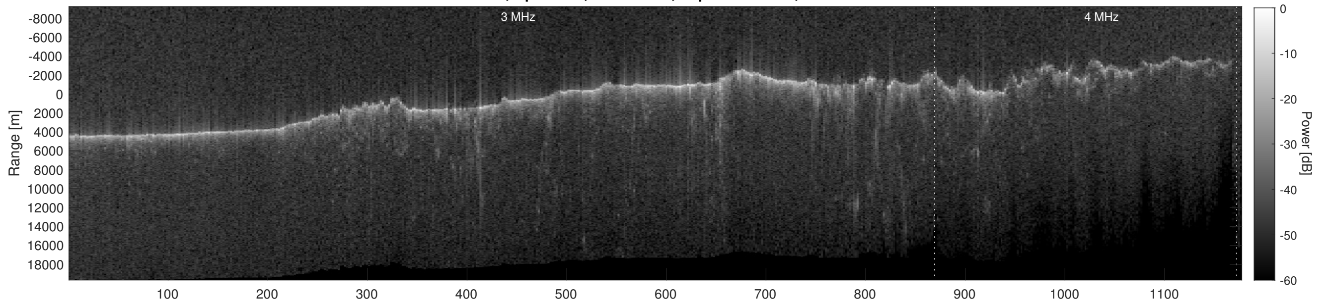
Orbit 9184, Depth-Corrected Cluttergram
