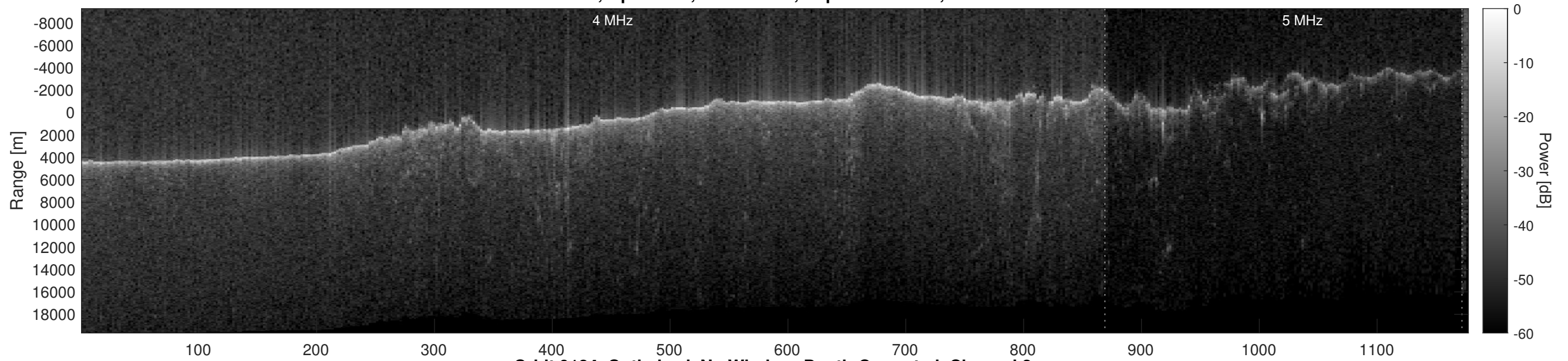
Orbit 9184, Optimized, No Window, Depth-Corrected, Channel 2
