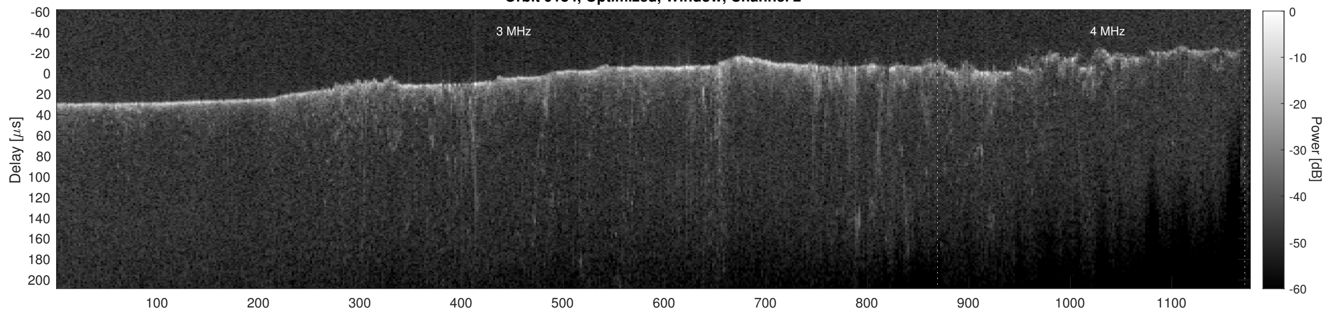
Orbit 9184, Cluttergram
