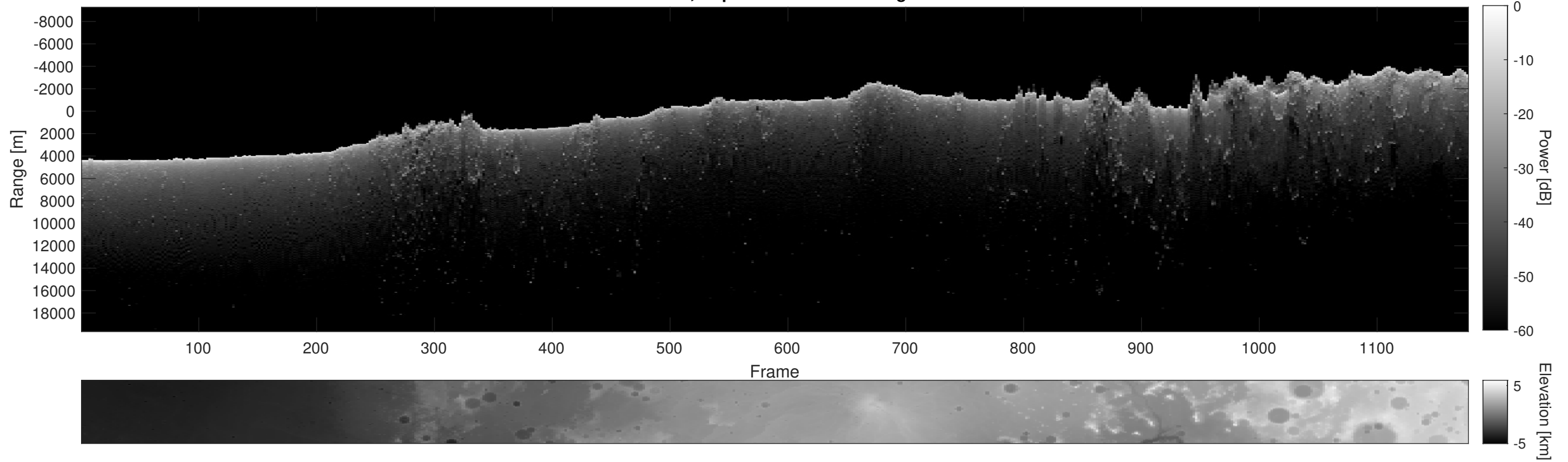
Orbit 9184, Depth-Corrected Cluttergram
