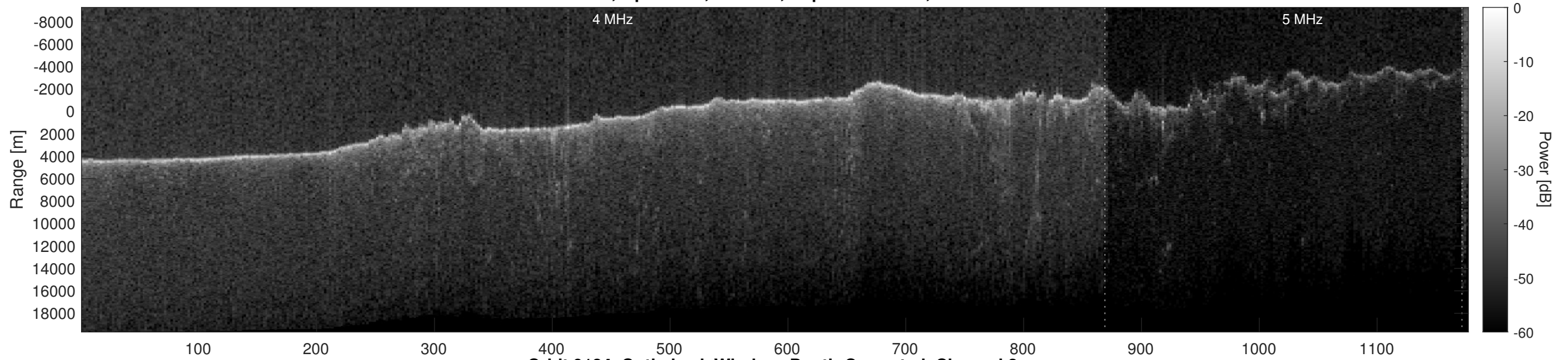
Orbit 9184, Optimized, Window, Depth-Corrected, Channel 2
