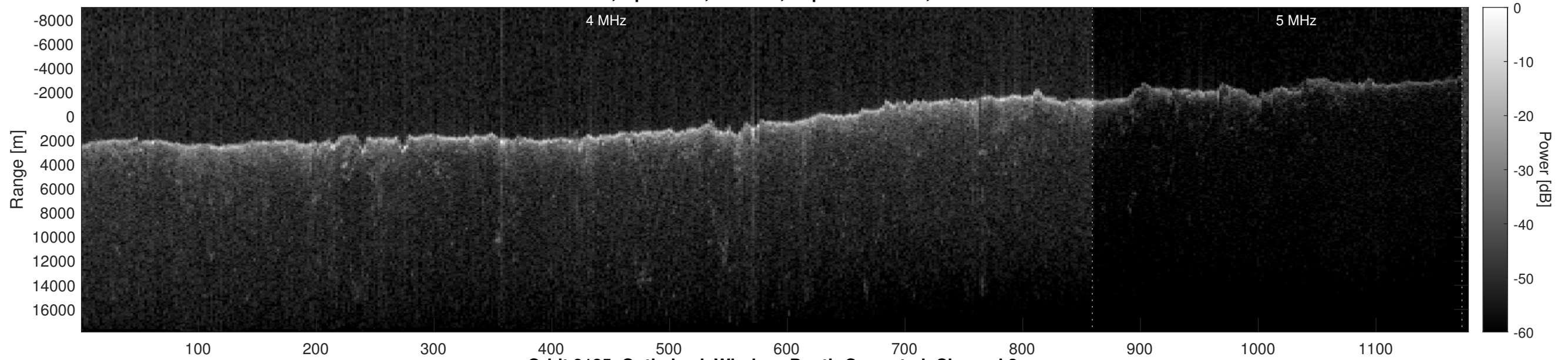
Orbit 9185, Optimized, Window, Depth-Corrected, Channel 2
