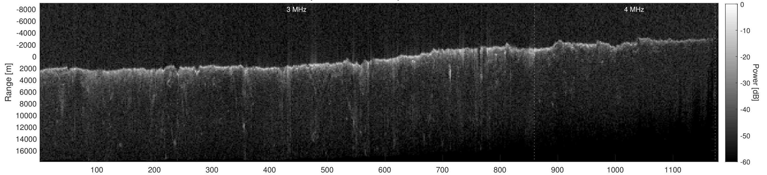
Orbit 9185, Depth-Corrected Cluttergram
