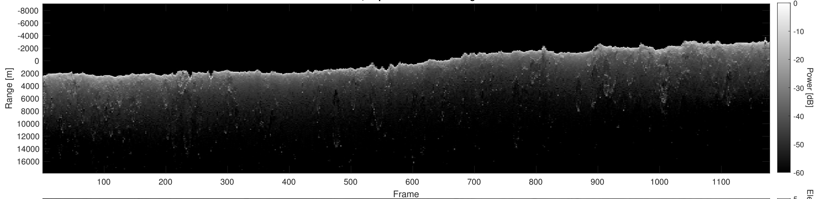
Orbit 9185, Depth-Corrected Cluttergram
