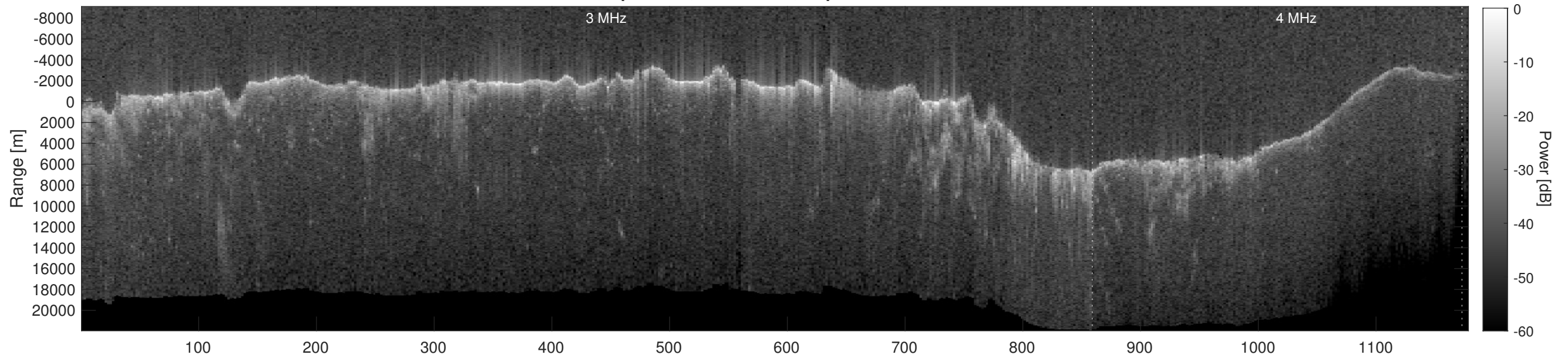
Orbit 9188, Depth-Corrected Cluttergram
