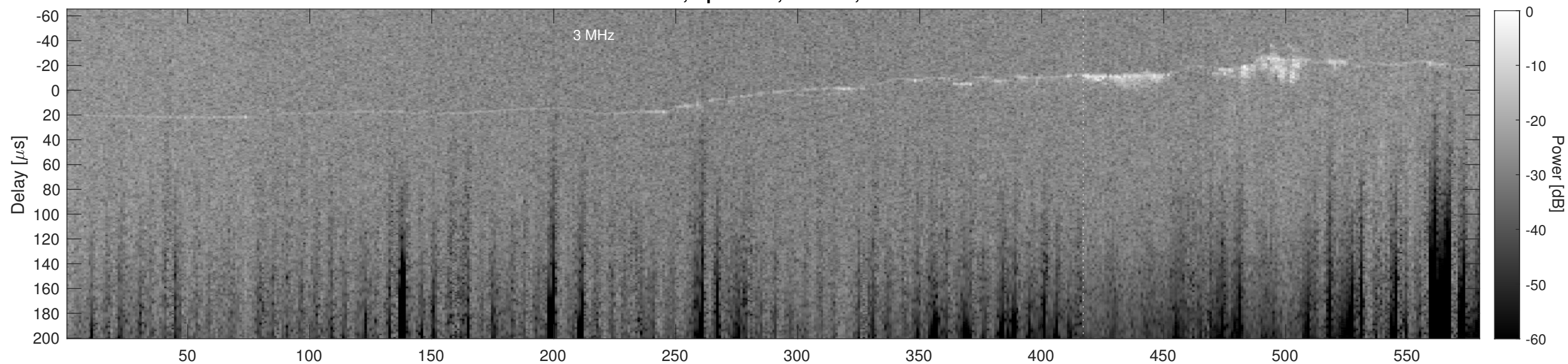
Orbit 9190, Cluttergram
