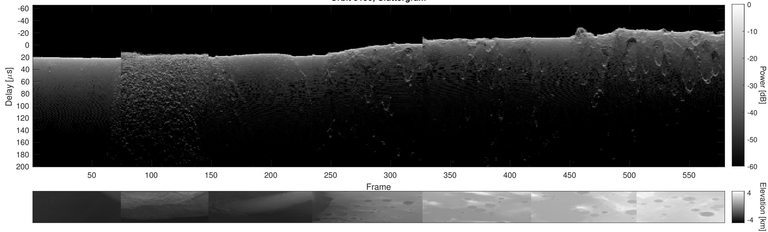
Orbit 9190, Cluttergram
