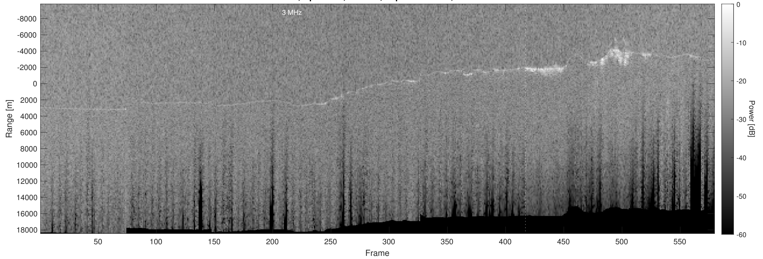
Orbit 9190, Optimized, Window, Depth-Corrected, Channel 2
