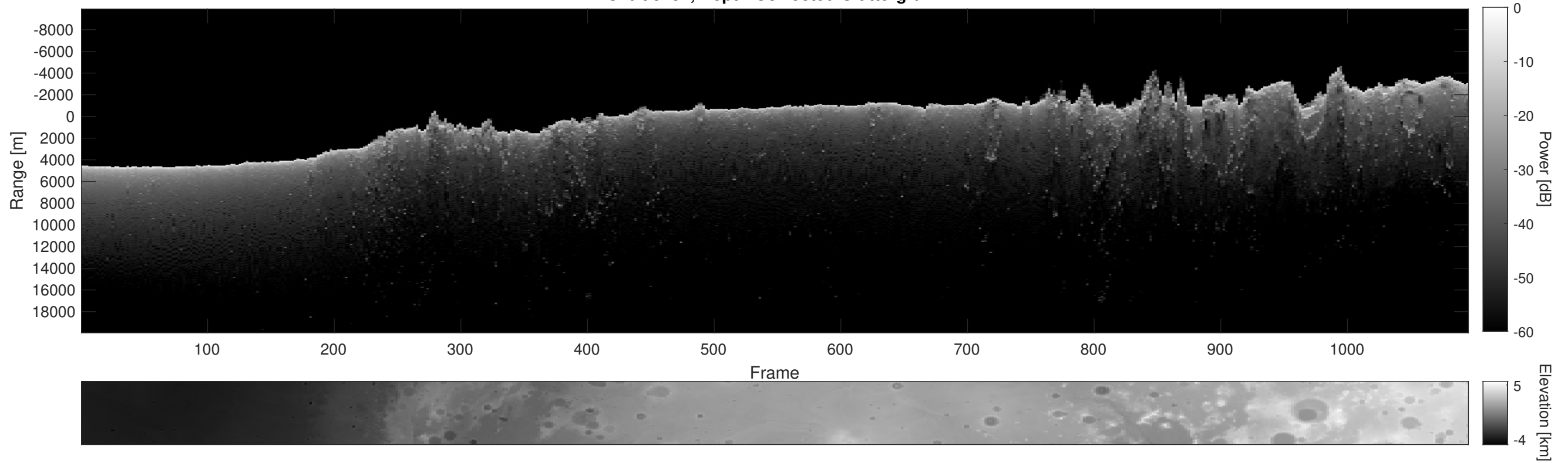
Orbit 9191, Depth-Corrected Cluttergram
