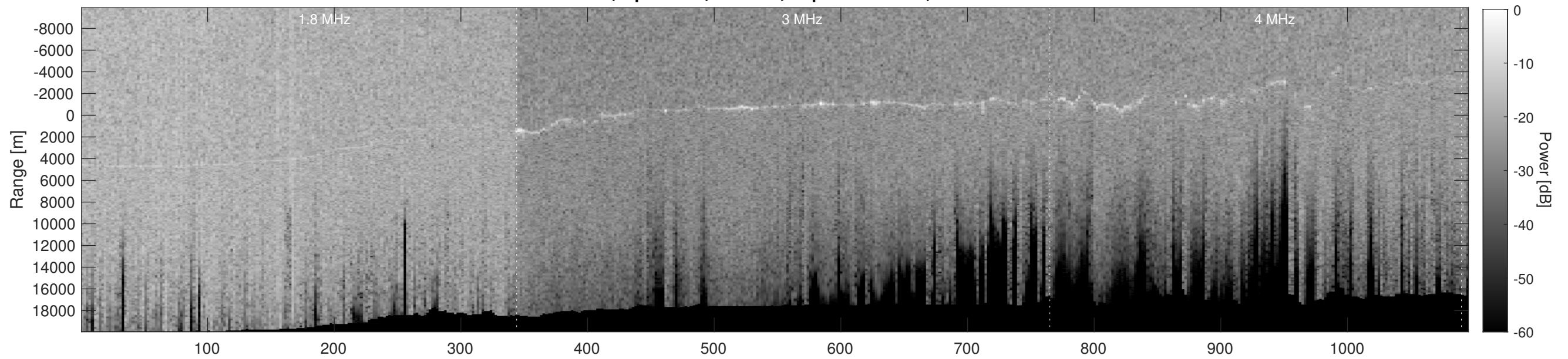
Orbit 9191, Depth-Corrected Cluttergram
