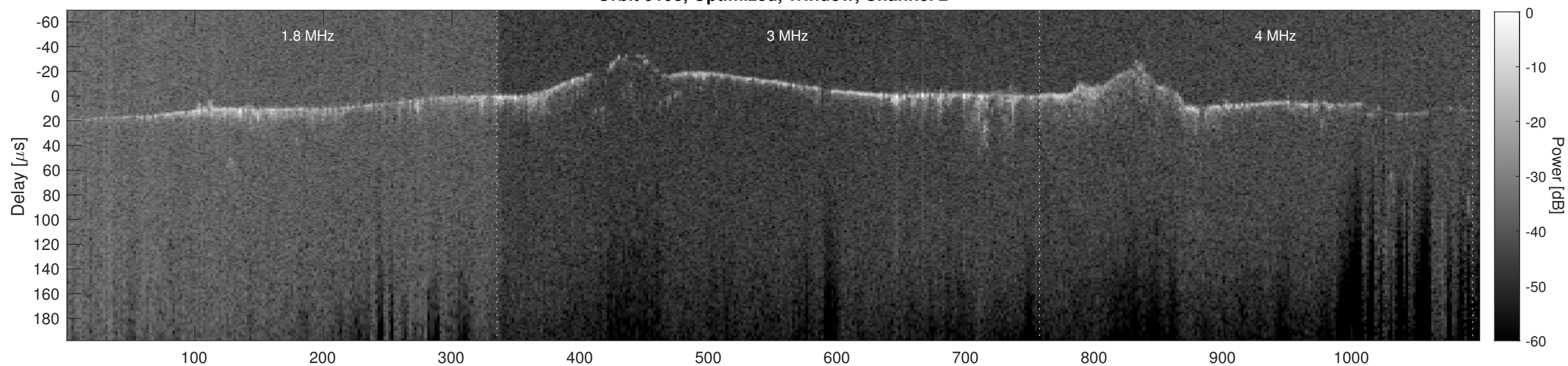
Orbit 9193, Cluttergram
