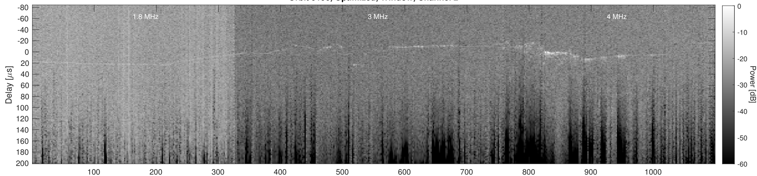
Orbit 9196, Cluttergram
