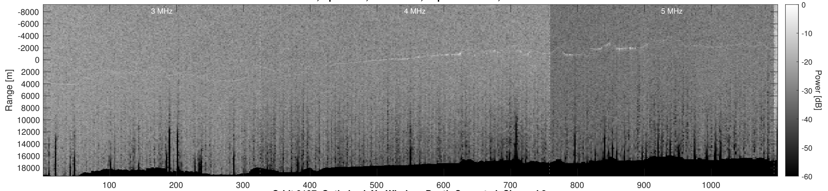
Orbit 9197, Optimized, No Window, Depth-Corrected, Channel 2
