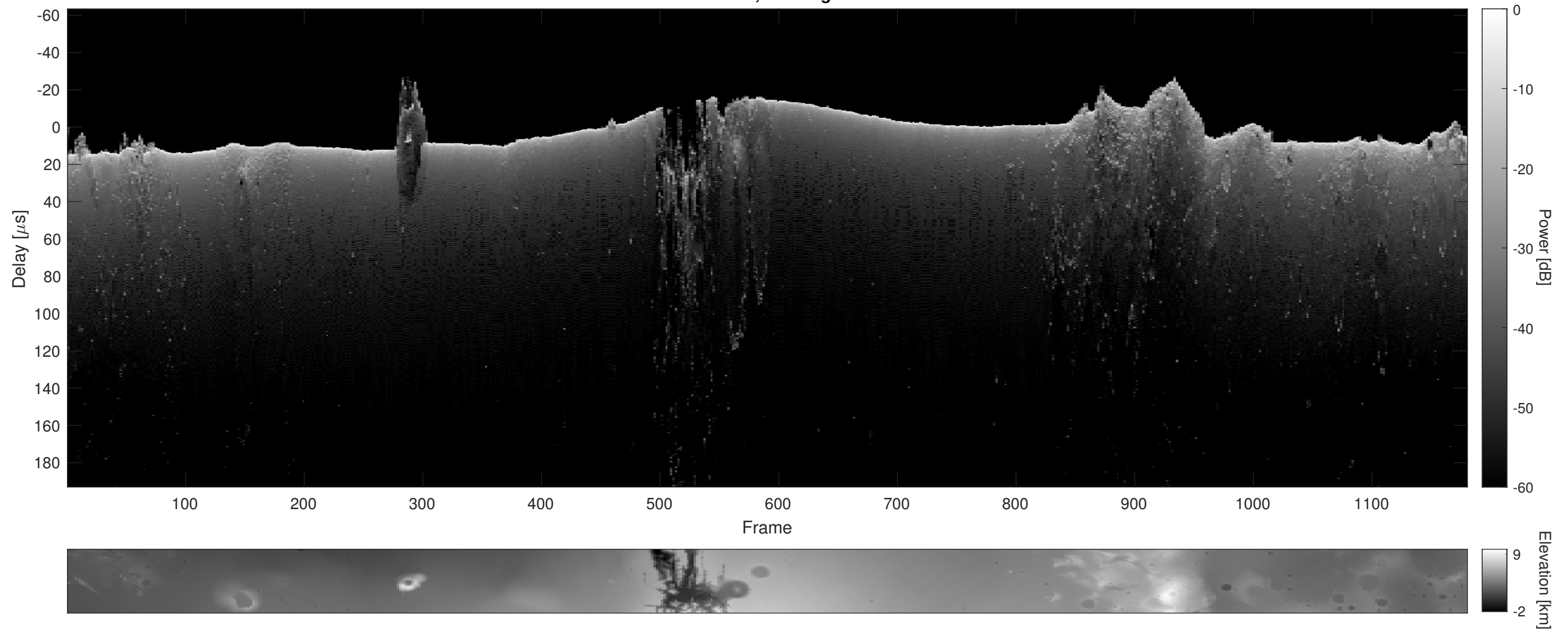
Orbit 9200, Cluttergram
